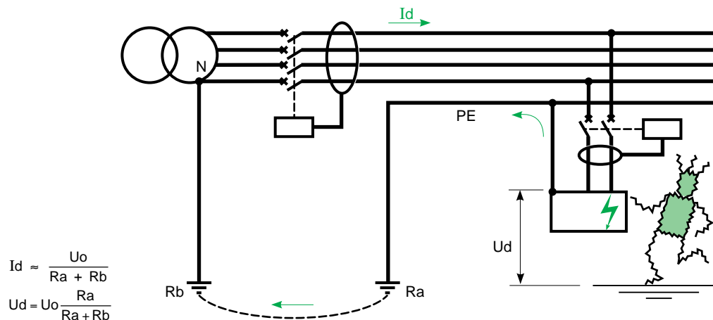
Fig. 10 : fault current and voltage in TT system.
