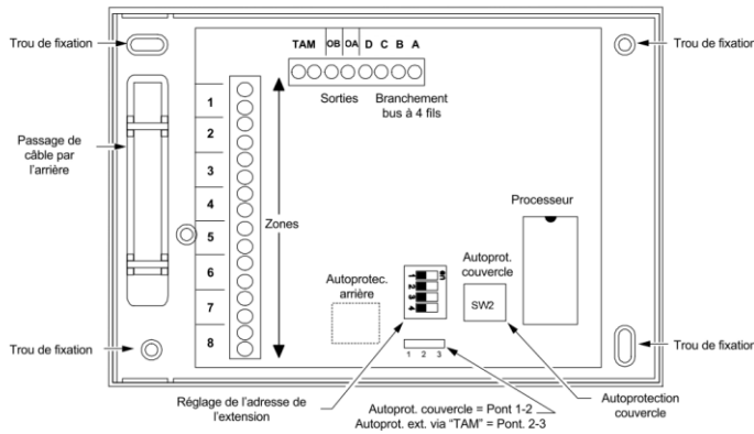
Figure 17. Extension CD9031S33
