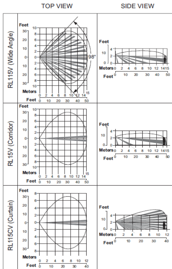
Figure 4. iWISE DT AM With ACT & Green Line G3 Lense and microwave Range
