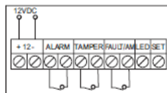
Figure 8. Terminal Wiring
