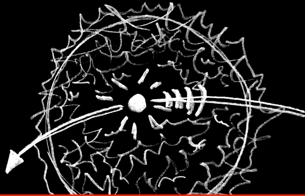
The Sun and Venus
